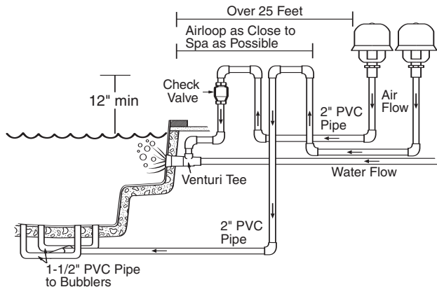
Diagram 2 - Long Run Installation (Over 25' from Spa)
