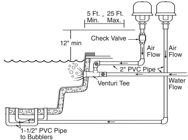
Diagram 1 - Typical Installation (5' - 25' from Spa)
